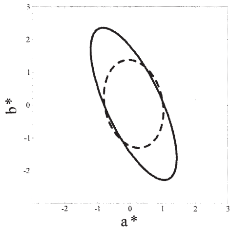
(a) CIE Gray color center
