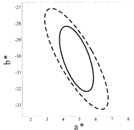
(e) CIE Blue color center
