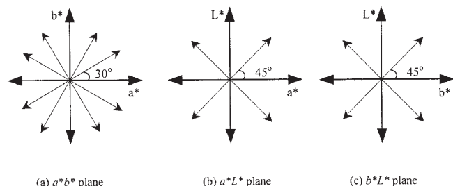
FIG. 1. Color stimuli distribution in CIELAB space. (a) a^*b^* plane; (b) a^*L^* plane; (c) b^*L^* plane.
