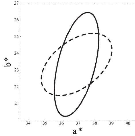
(b) CIE Red color center
